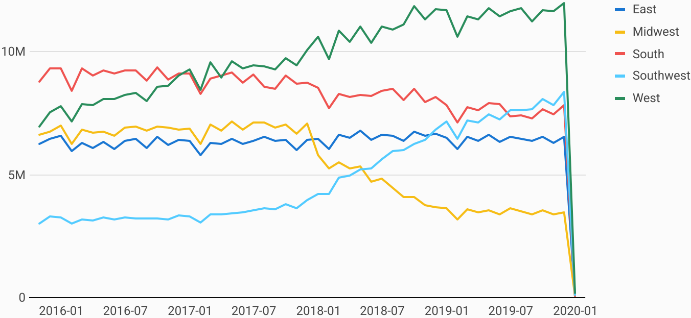
CountDistinct of Cust Key by Product Family and Store Region
